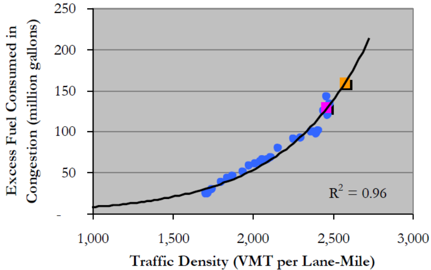
Figure 11: Correlation between Traffic Density and Excess Fuel Consumption
