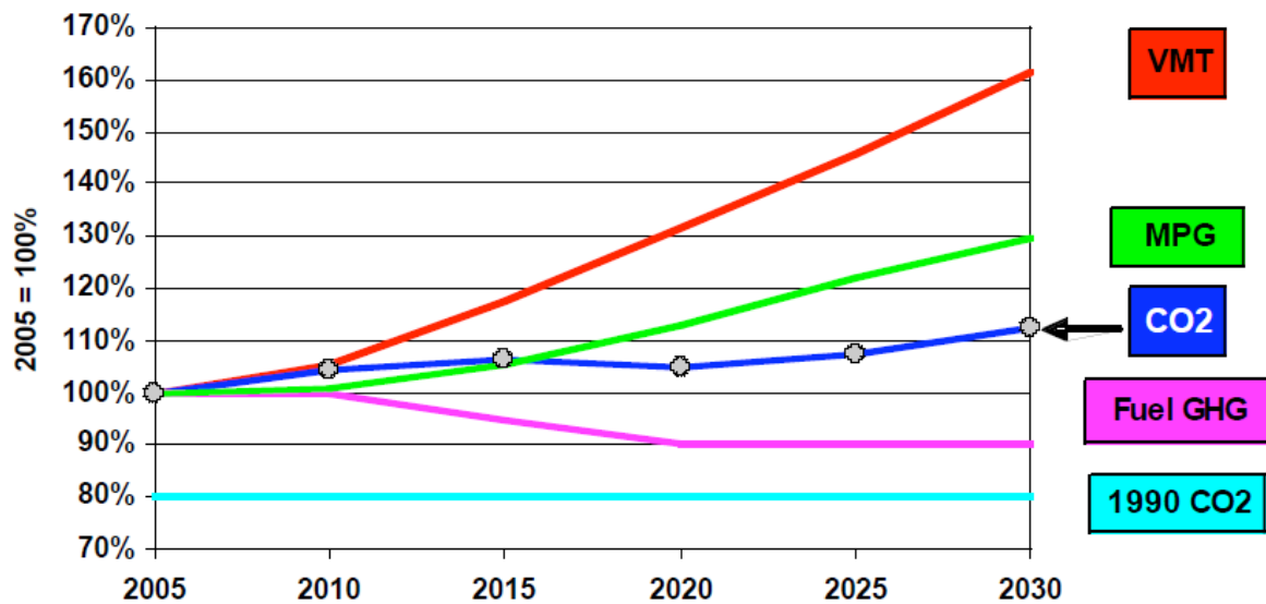
Figure 1: Projected Growth in CO 2 Emissions from Cars and Light Trucks Assuming Stringent Nationwide Vehicle and Fuel Standards*
