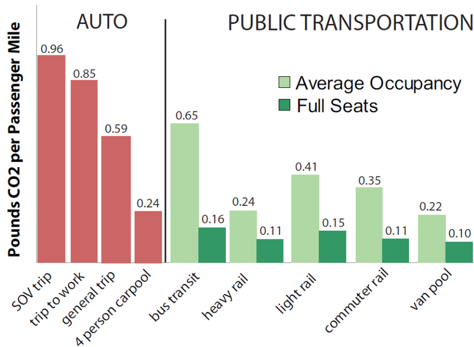
Figure 2: Estimated CO 2 Emissions per Passenger Mile for Average and Full Occupancy
